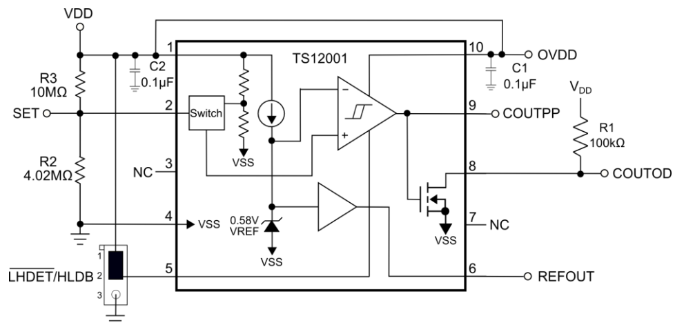
Figure 2. TS12001 Voltage Detector Circuit
