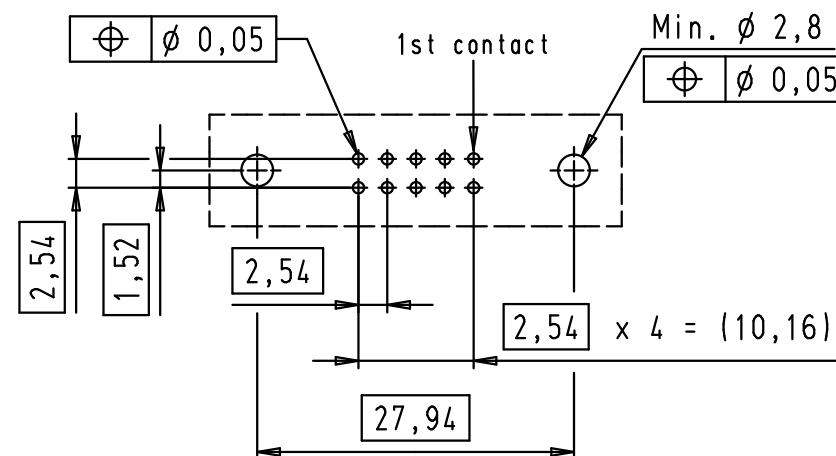
PCB layout, component side
