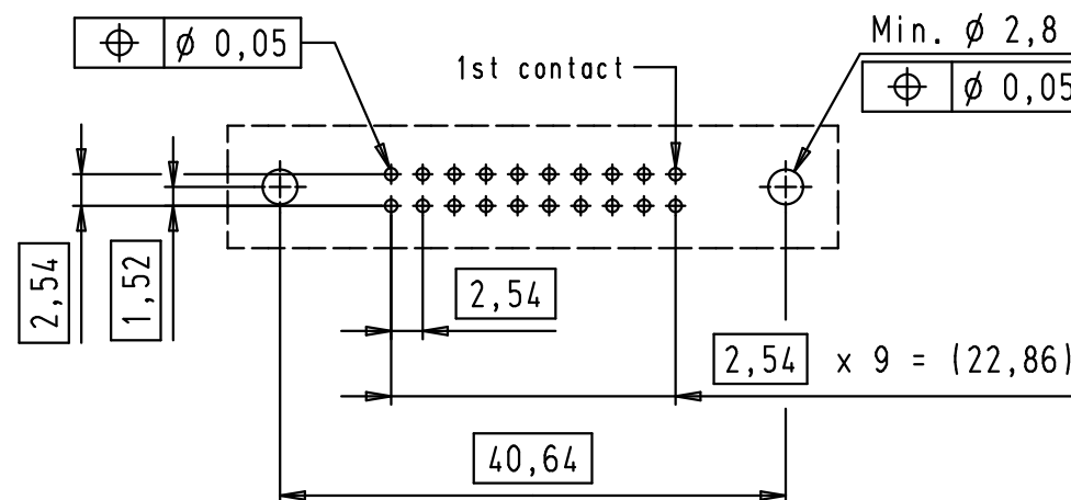
PCB layout, component side
