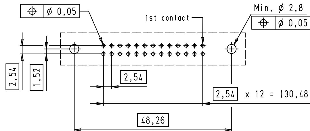
PCB layout, component side
