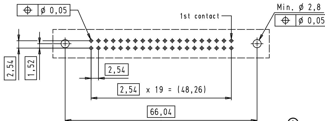
PCB layout, component side
