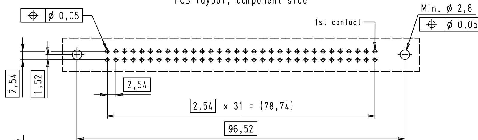
PCB layout, component side
