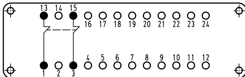
Schaltplan/wiring diagram
