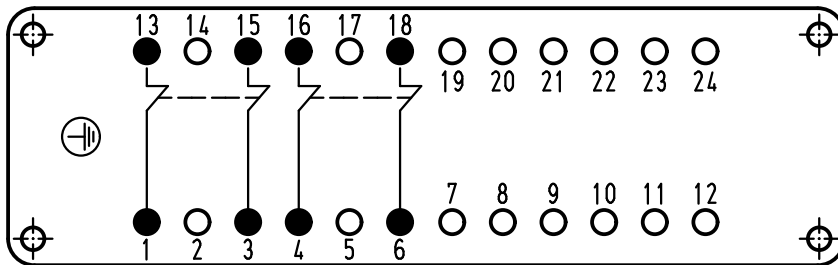
Schaltplan/wiring diagram
