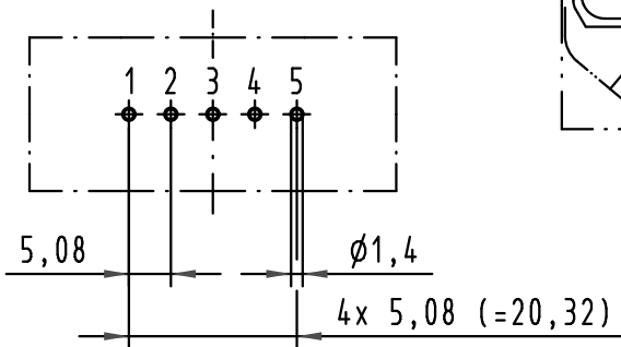
PCB-Layout 1:1
