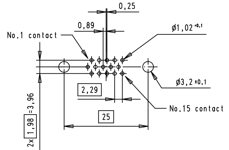
Printed layout component side
