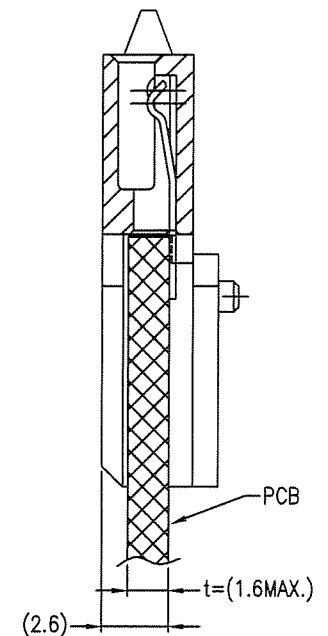
SECT.Y-Y
