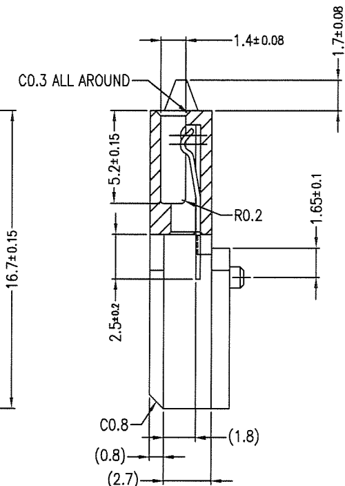
SECT.X-X
