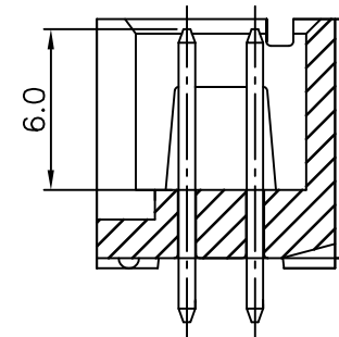
SECTION A-A WITHOUT CAP
