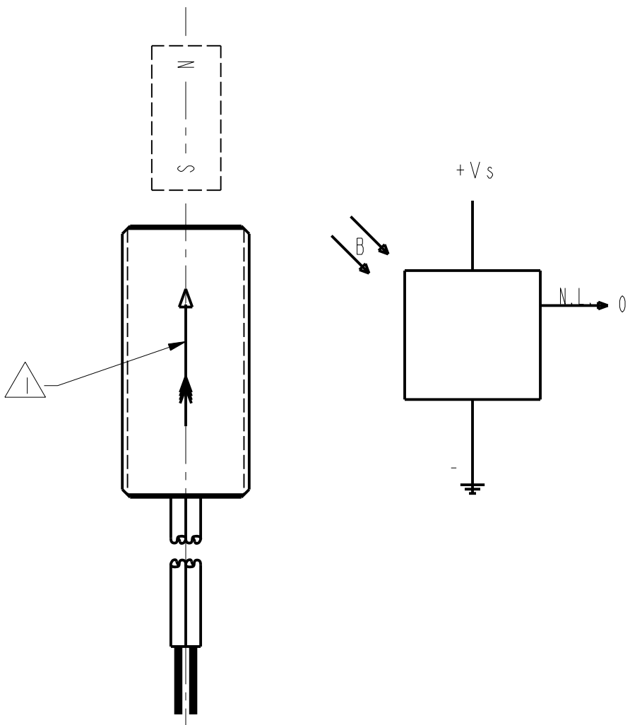
FIG. 2 OPERATE
