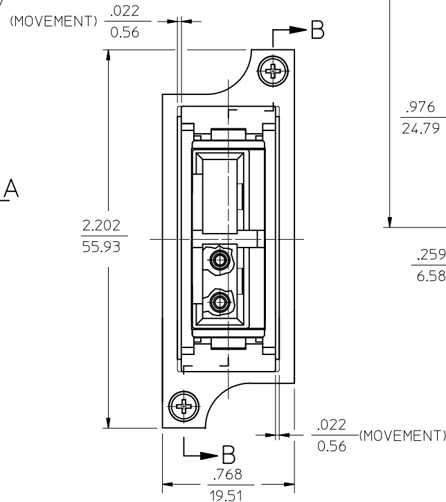
VIEW A RECOMMENDED MOUNTING HOLES
