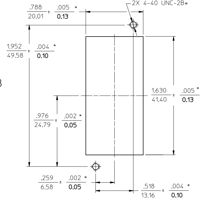
VIEW A RECOMMENDED MOUNTING HOLES
