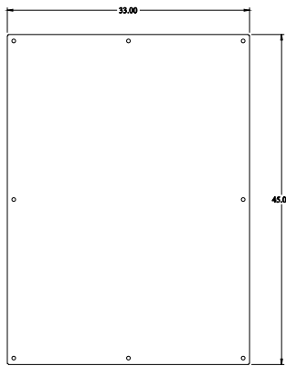
INNER PANEL
