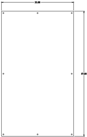
INNER PANEL
