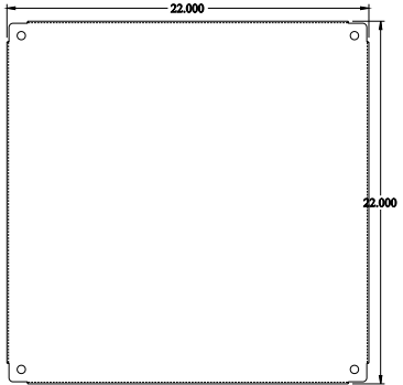
INNER PANEL
