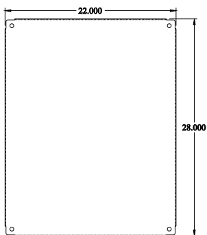
INNER PANEL
