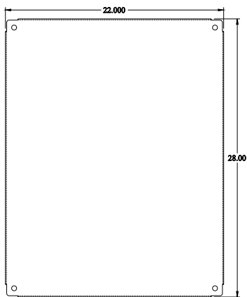
INNER PANEL
