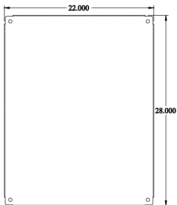
INNER PANEL
