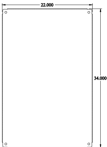
INNER PANEL
