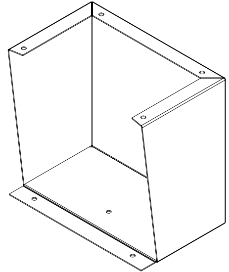
ISOMETRIC VIEW
