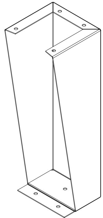
ISOMETRIC VIEW
