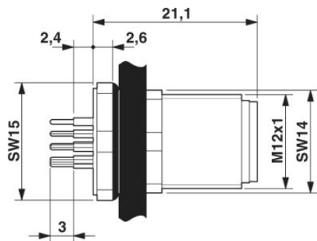
Dimensioned drawing
