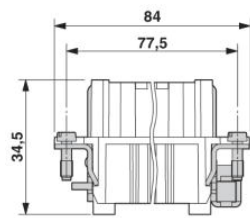
Female insert
