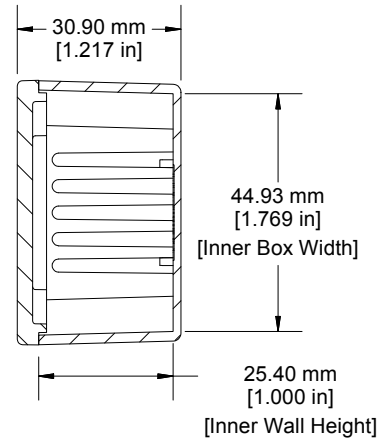
Top View Looking Inside Box
