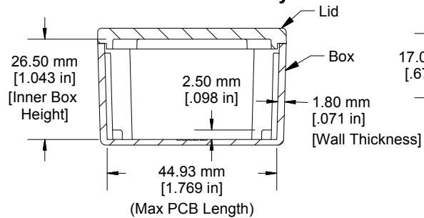
SECTION B-B Side View of Assembly
