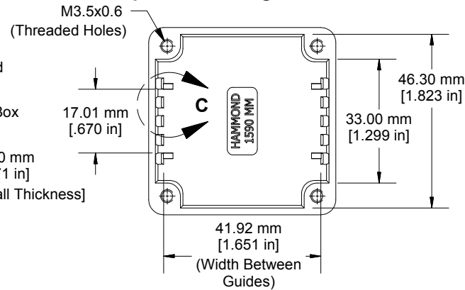
DETAIL C Top View - Interior Features
