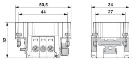
Male insert
