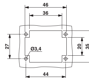
Panel cutout
