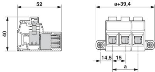
Dimensioned drawing
