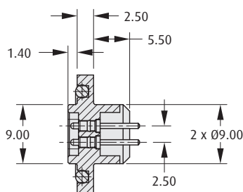
PC Tail
