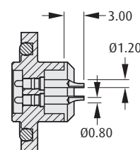
Solder Cup
