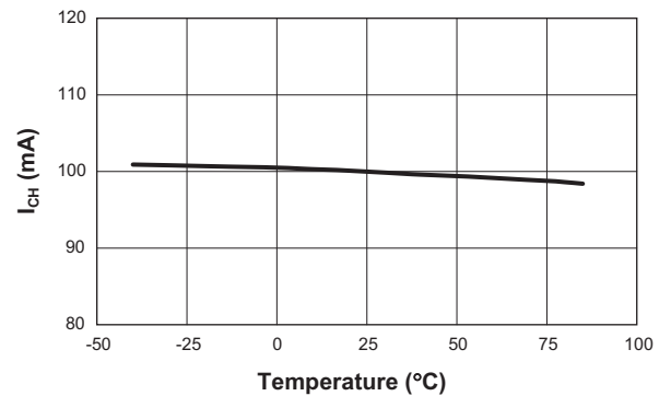
Preconditioning Charge Current vs. Temperature (SETH; SETH = 3.83k \Omega )
