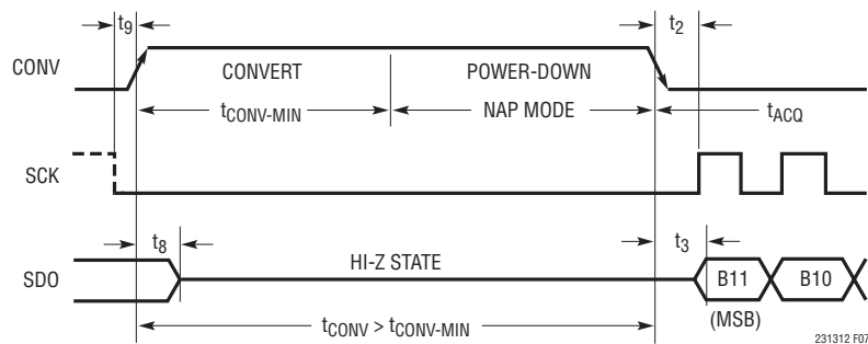
Figure 7. LTC2313-12 Nap Mode Power-Down Following Conversion for t_{CONV} > t_{CONV-MIN}
