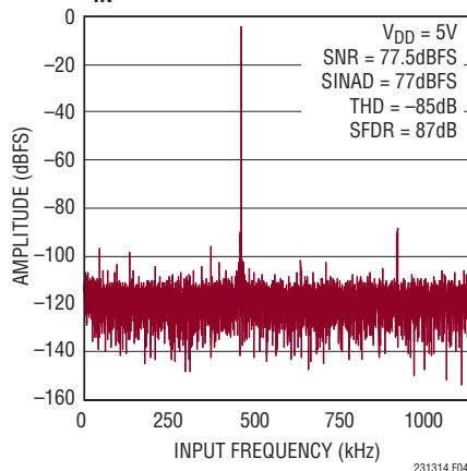
16k Point FFT, f_S = 2.5\text{MSPS} f_{\text{IN}} = 497\text{kHz}
