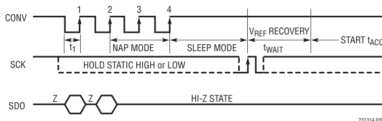
Figure 9. LTC2313-14 Entering/Exiting Sleep Mode
