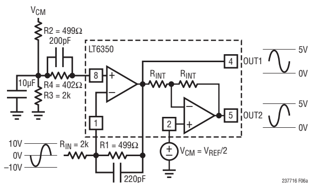
Figure 6a. LT6350 Converting a ±10V Single-Ended Signal to a ±5V Differential Input Signal
