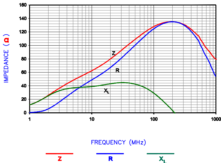
|Z| , R, AND X vs. FREQUENCY
