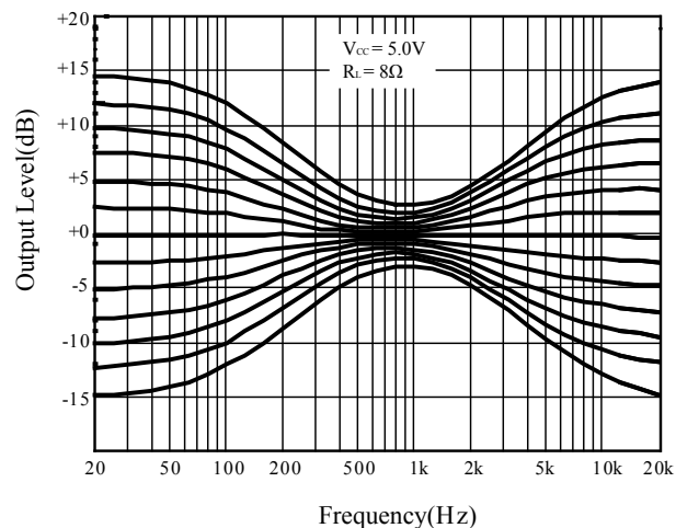
Figure 12 Bass and Treble Response vs. Frequency
