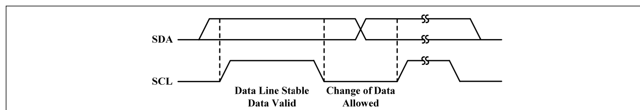
Figure 14 Bit transfer
