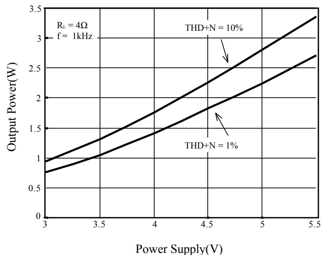
Figure 10 Output Power vs. Power Supply
