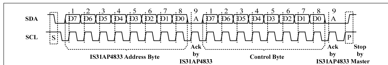
Figure 15 Writing to IS31AP4833
