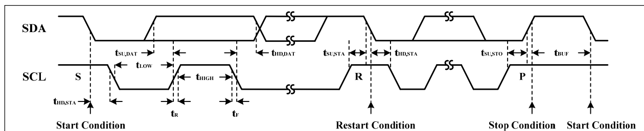
Figure 13 Interface timing
