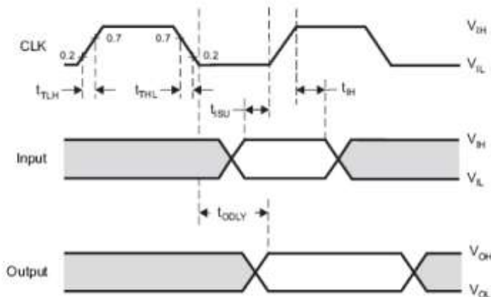
Figure 11 SDIO Timing
