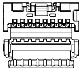
8 CIRCUIT RECEPTACLE POLARIZATION OPTION C
