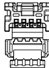
4 CIRCUIT RECEPTACLE POLARIZATION OPTION D
