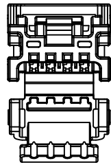
4 CIRCUIT RECEPTACLE BRIDGED POLARIZATION OPTION A
