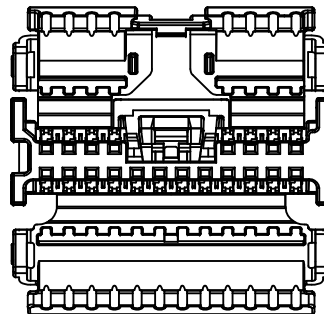
16 CIRCUIT RECEPTACLE WITH LOCK BRIDGE POLARIZATION OPTION C
