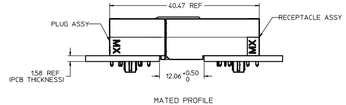
MATED PROFILE
