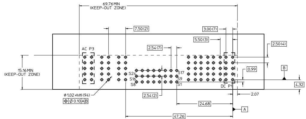
RECOMMENDED PC BOARD LAYOUT & KEEP-OUT ZONE
