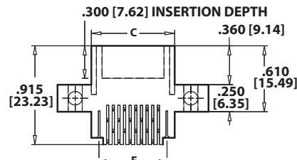
(S) MOUNTING SHOWN
