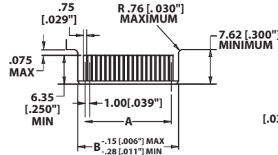
CARD LAYOUT
