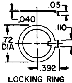
LOCKING RING
