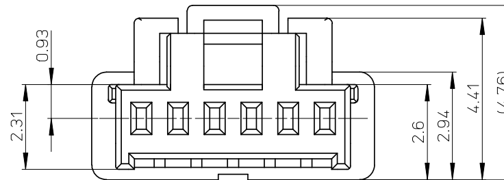
VIEW "D"
