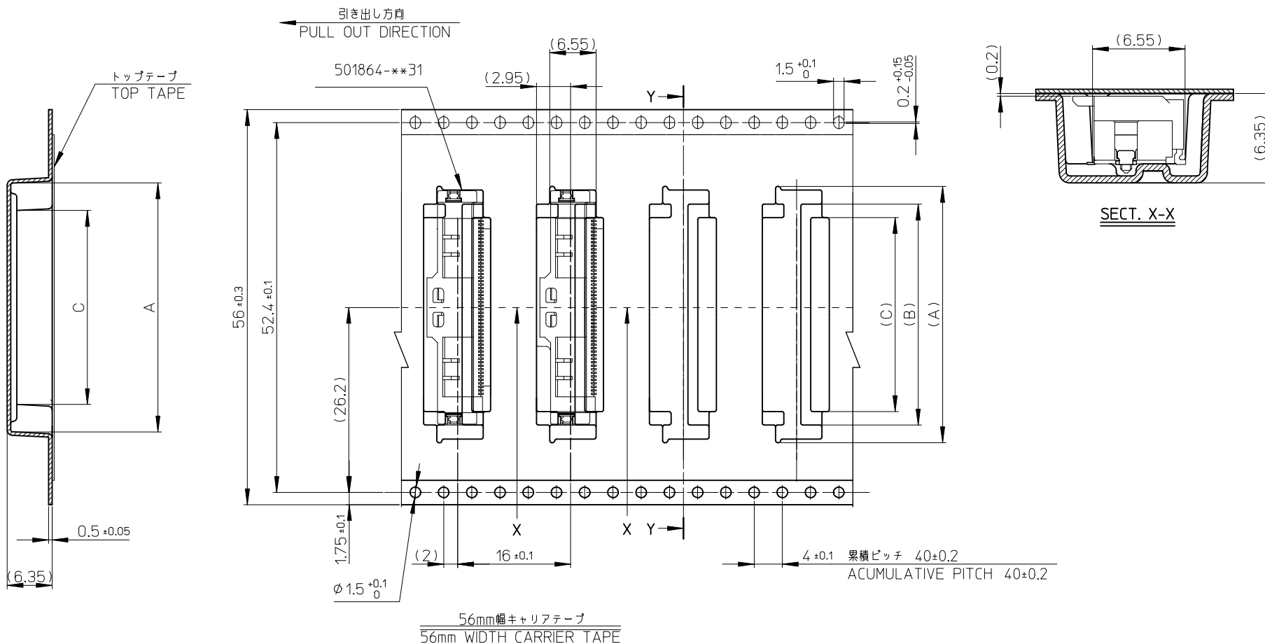
SECT. Y-Y
