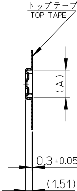
SECTION Y-Y
