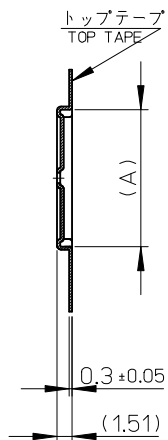
SECTION Y-Y
