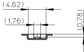
SECTION X-X
