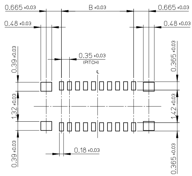
RECOMMENDED P.W. BOARD PATTERN LAYOUT
