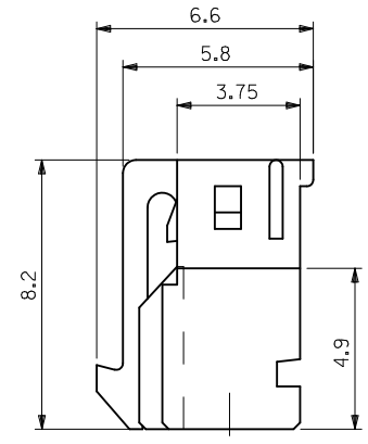
VIEW "H"
