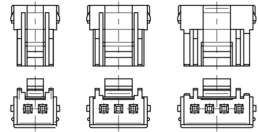
LAYOUT OF EACH CKTS.
