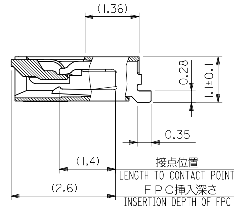
断面 W-W SECT. W-W (Scale 15:1) 偶数極 (EVEN CIRCUIT)
