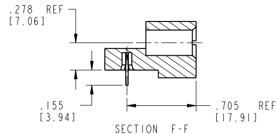
SECTION F-F
